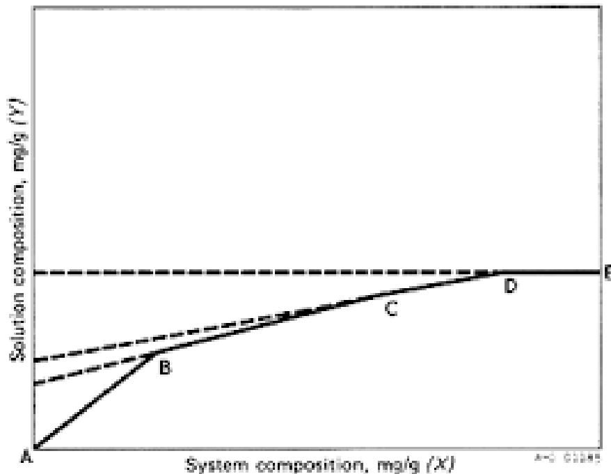
Fig.3 . TYPICAL PHASE SOLUBILITY DIAGRAM
